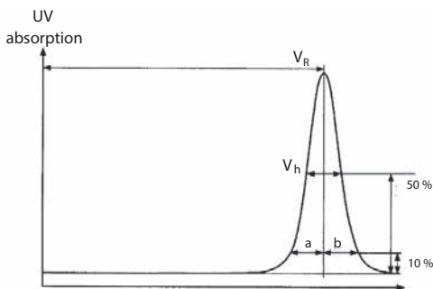
Fig 1. Example showing results obtained from the column evaluation method described above
